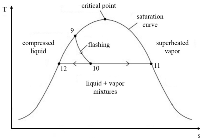
Fig. 4. Flashing on temperature–entropy diagram. Note: depending on each case, state 9 can correspond to saturated liquid, as represented in this figure, but also as compressed liquid, or a liquid–vapor mixture.
